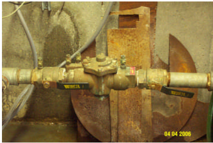
REDUCED PRESSURE ZONE BACKFLOW ASSEMBLY
